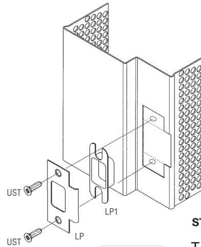
TYPICAL T-STRIKE ASSEMBLY
